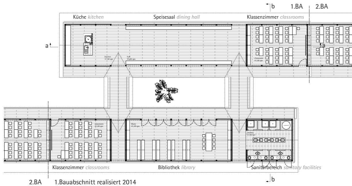
Grundriss ground floor plan
